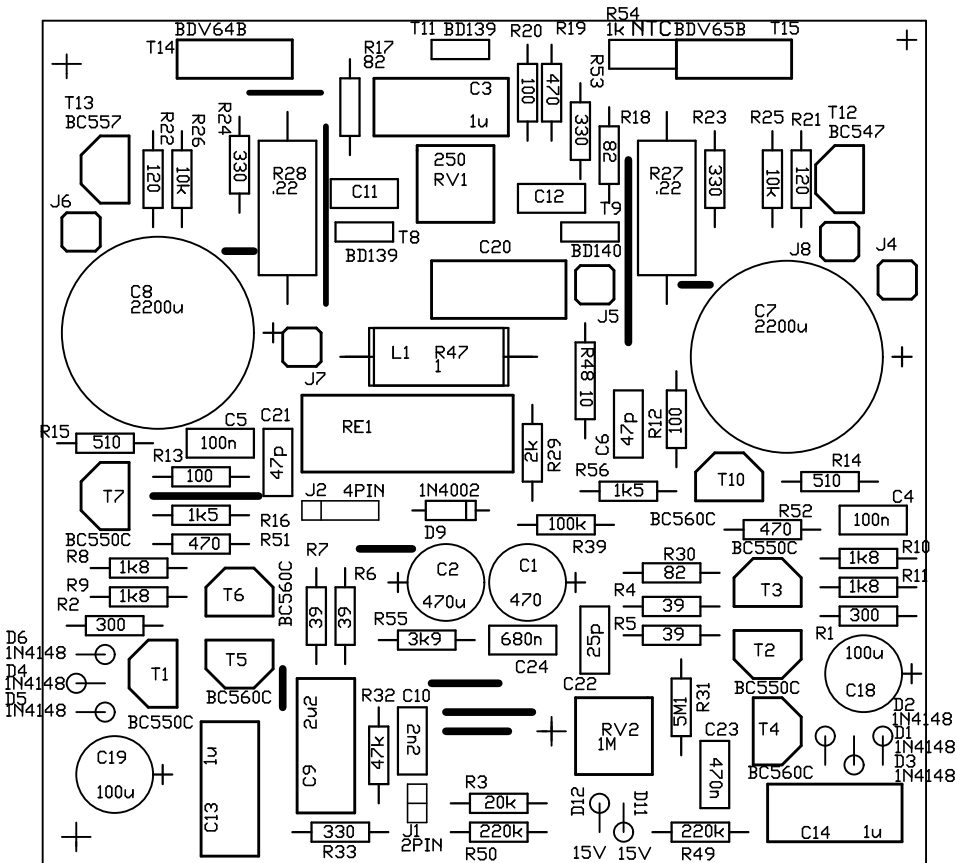
DRIVER2 Top Overlay
