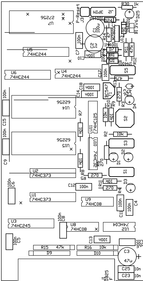
EPROM Top Overlay
